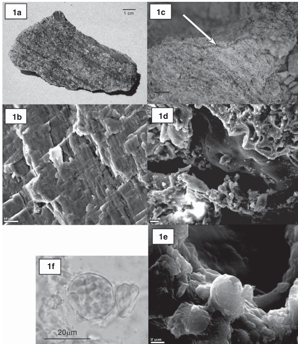
Fig. 4 Micro-organisms associated with the impact-shocked gneiss at the Haughton impact crater. These types of microhabitats serve as analogs for the types of microhabitats explorers would search for on Mars. 1a. A piece of unshocked gneiss, also seen under Scanning Electron Microscopy (SEM) in (1b). Note that it contains few access points for microbial colonization. 1c shows a sample of shocked gneiss containing a coherent band of cyanobacterial endolithic growth (arrow). The organism inhabiting these rocks is the desiccation and radiation resistant cyanobacterium, Chroococidiopsis sp. 1 d shows a typical field of view in shocked rocks under SEM illustrating the presence of micro-factures and entry points for microbial colonization of the shocked microhabitats. 1e shows an SEM of a single Chroococidiopsis cell occupying an impact-induced micro-fracture. 1f shows a colony of cells inside their sheath under light microscopy. SEM images were obtained back in the UK. The visible micrograph was obtained in the habitat after the EVA.
