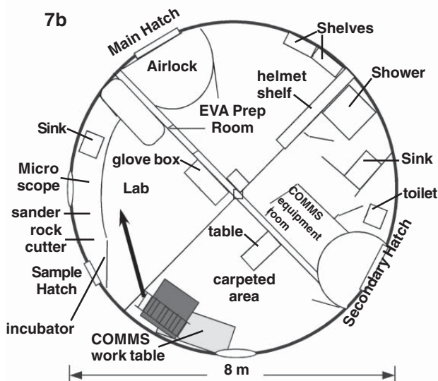
Fig. 7 Microscopy was accomplished in the lower deck laboratory (7a). In 7b the configuration of the laboratory on the lower deck of the habitat is shown with the locations of some instruments. The bold arrow indicates the direction of the view in Figure 7a.
